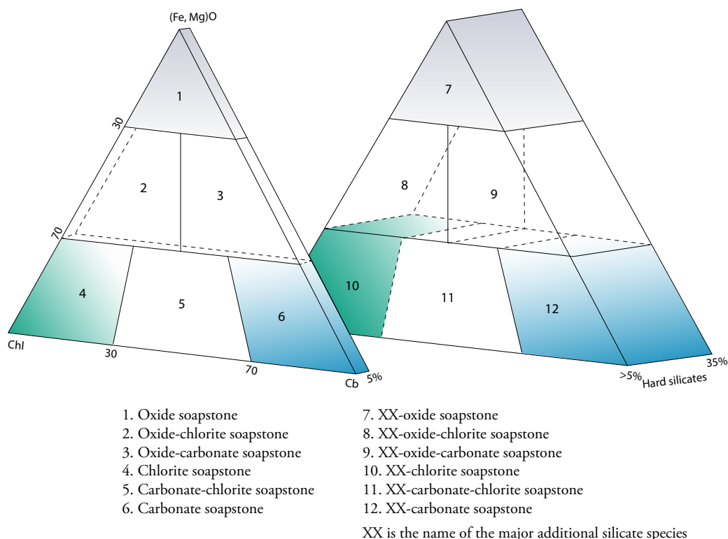
Figure 2. Designation of soapstone according to the relative quantities of oxide (O), chlorite (Ch), and carbonate (C), and the volumes of hard silicates. According to Huhta (2019).
